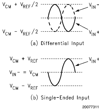
FIGURE 2. Expected Input Signal Range
